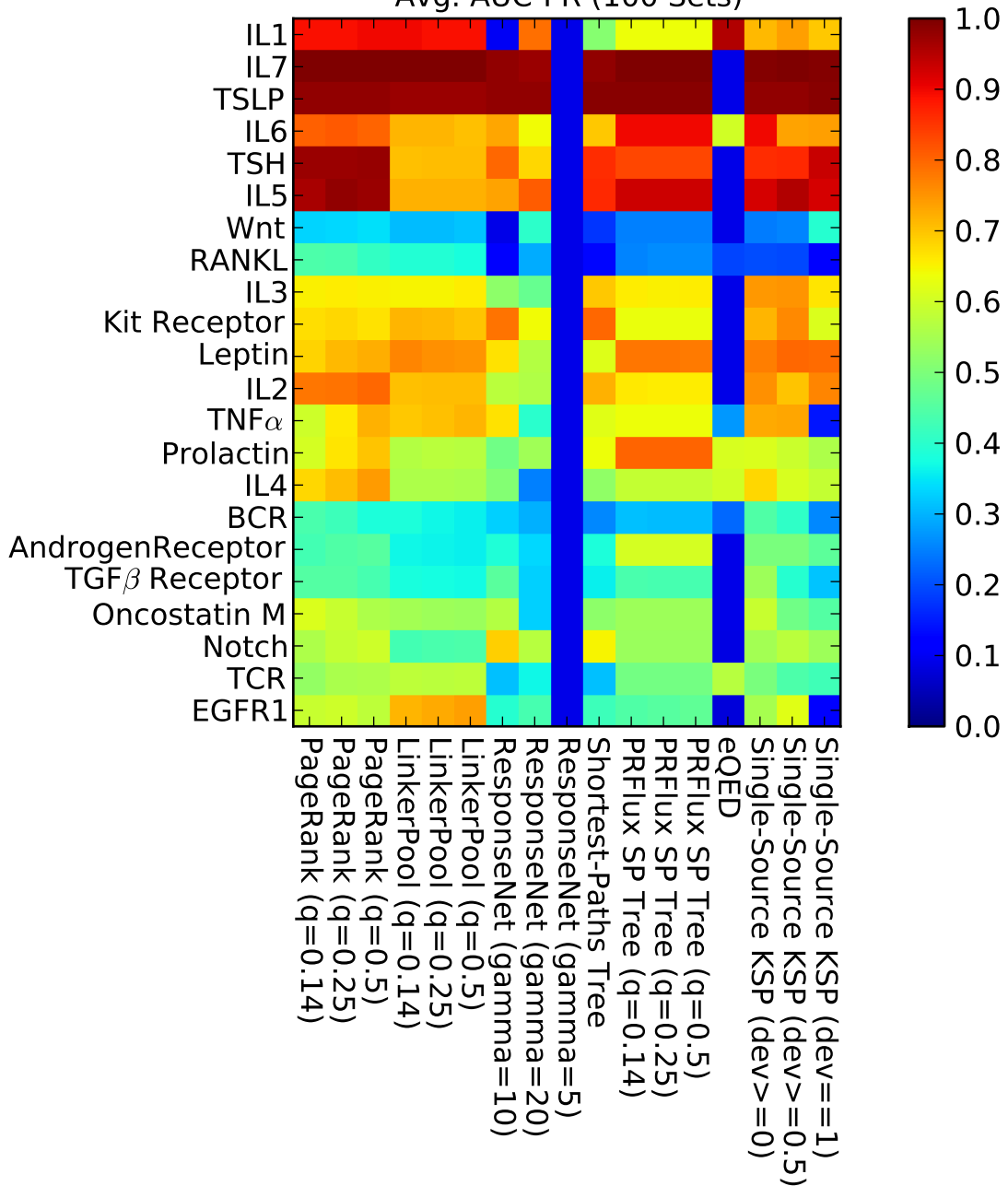
NetPath TFpool Avg. AUC-PR (100 Sets)
