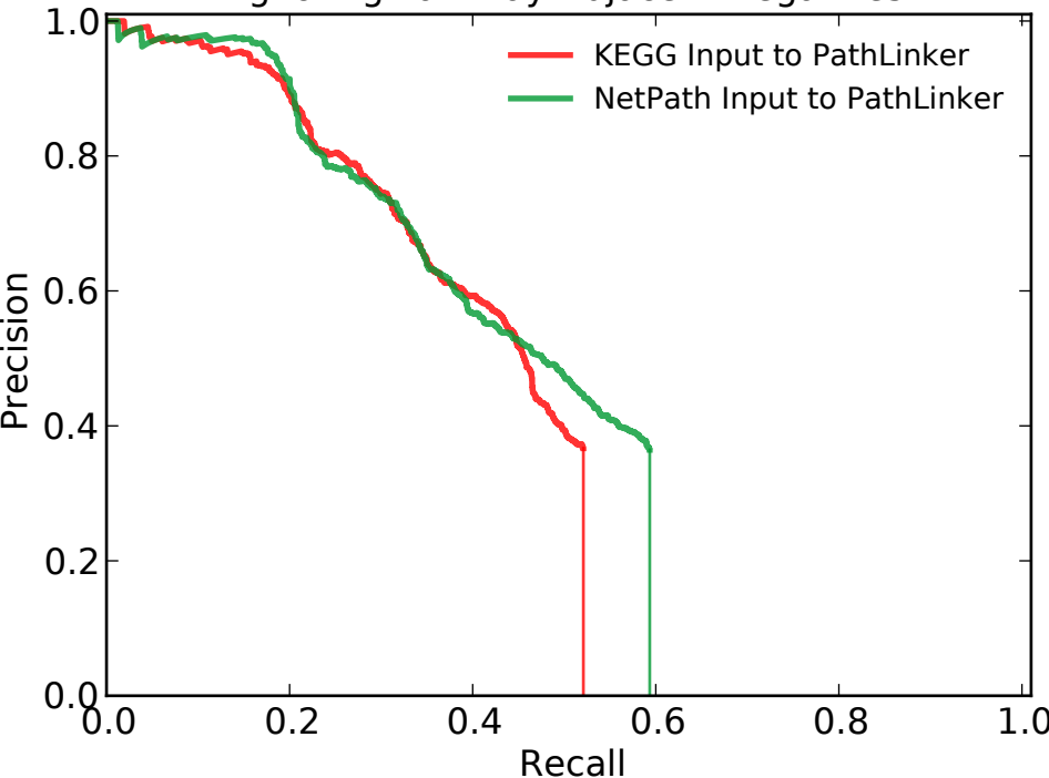
Interactions in the Aggregate KEGG + NetPath Pathway Recon. Ignoring Pathway-Adjacent Negatives
