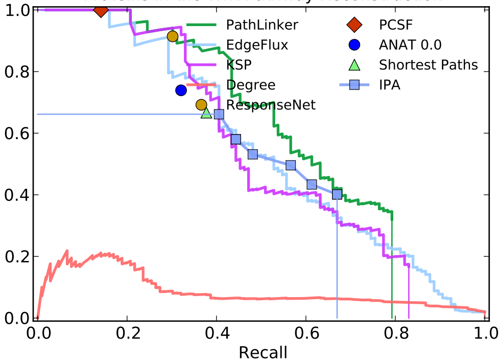
Proteins in the Wnt Pathway Reconstruction
