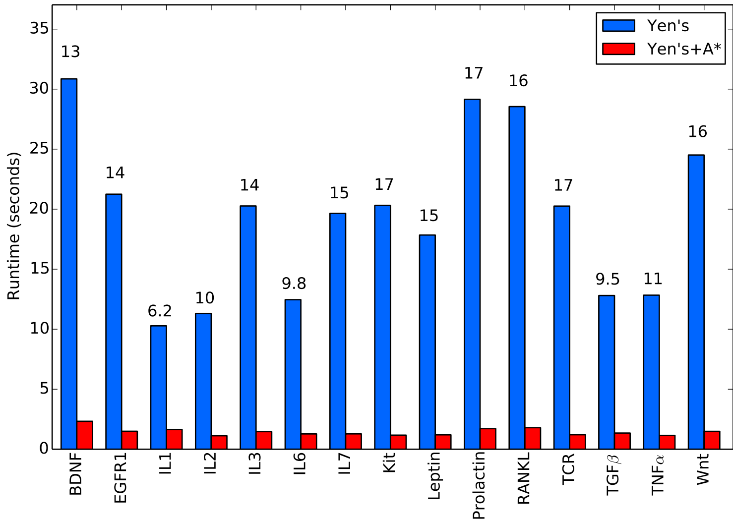
Runtime for k = 200
