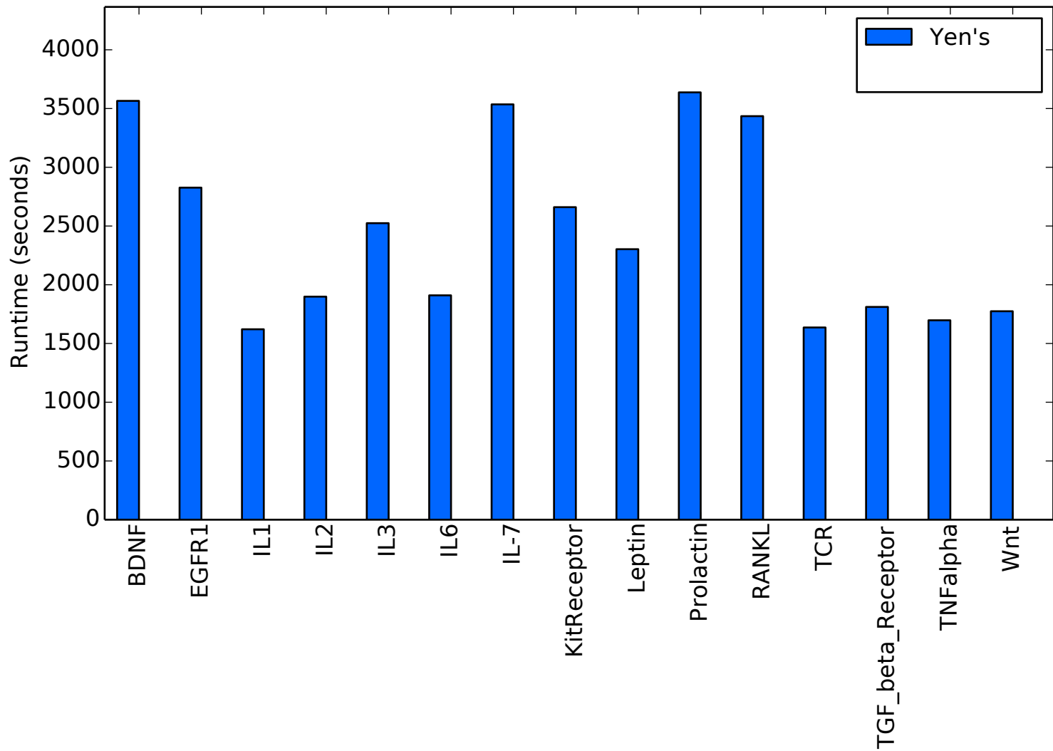
Runtime for k = 20000
