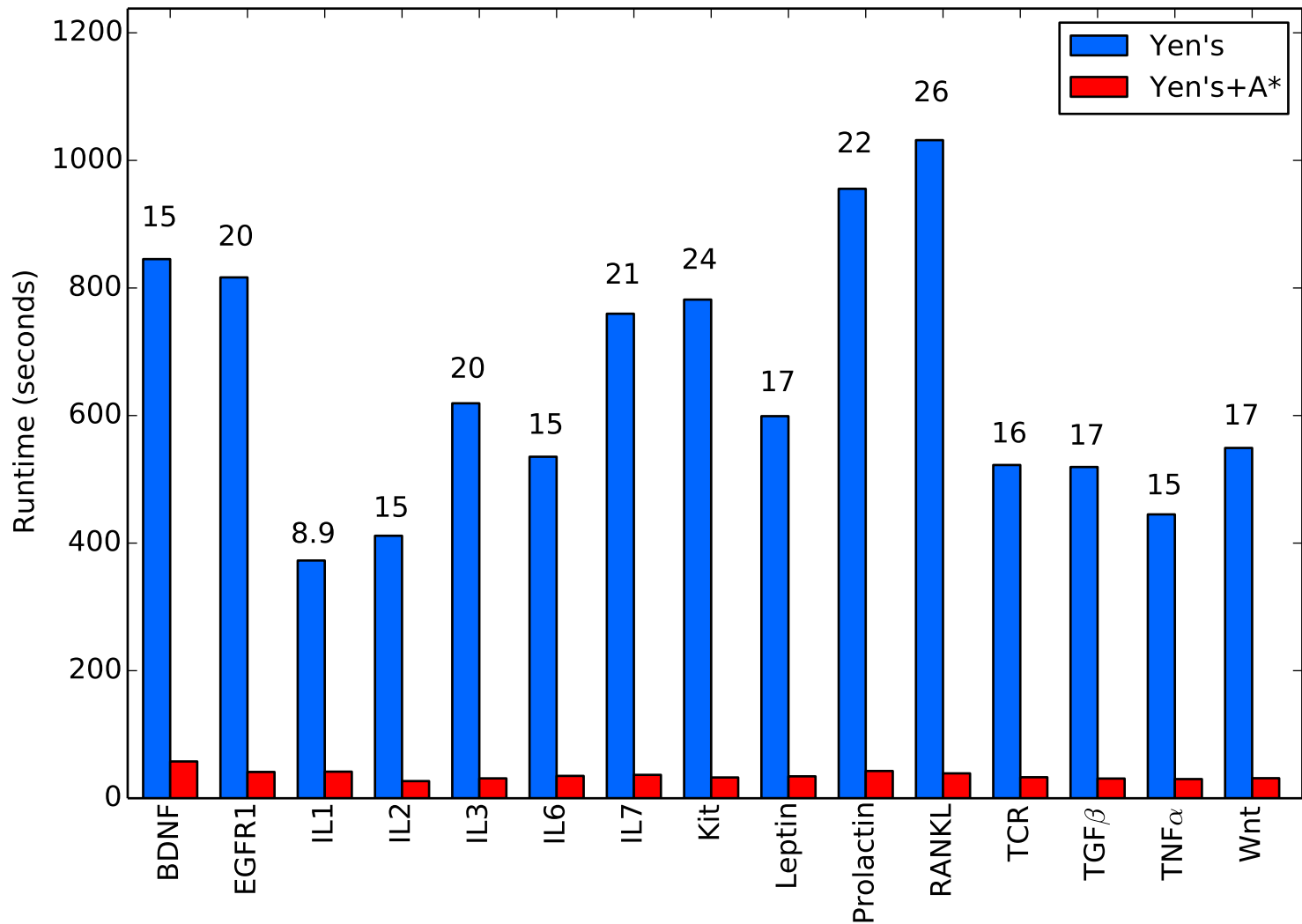
Runtime for k = 5000
