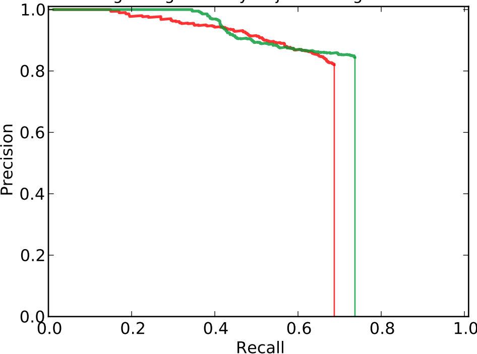
Proteins in the Aggregate KEGG + NetPath Pathway Recon. Ignoring Pathway-Adjacent Negatives
