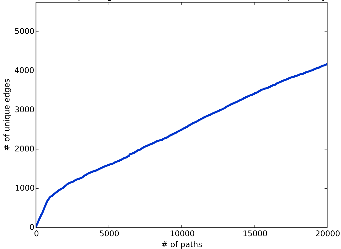
# of unique edges in the reconstruction of the BDNF pathway
