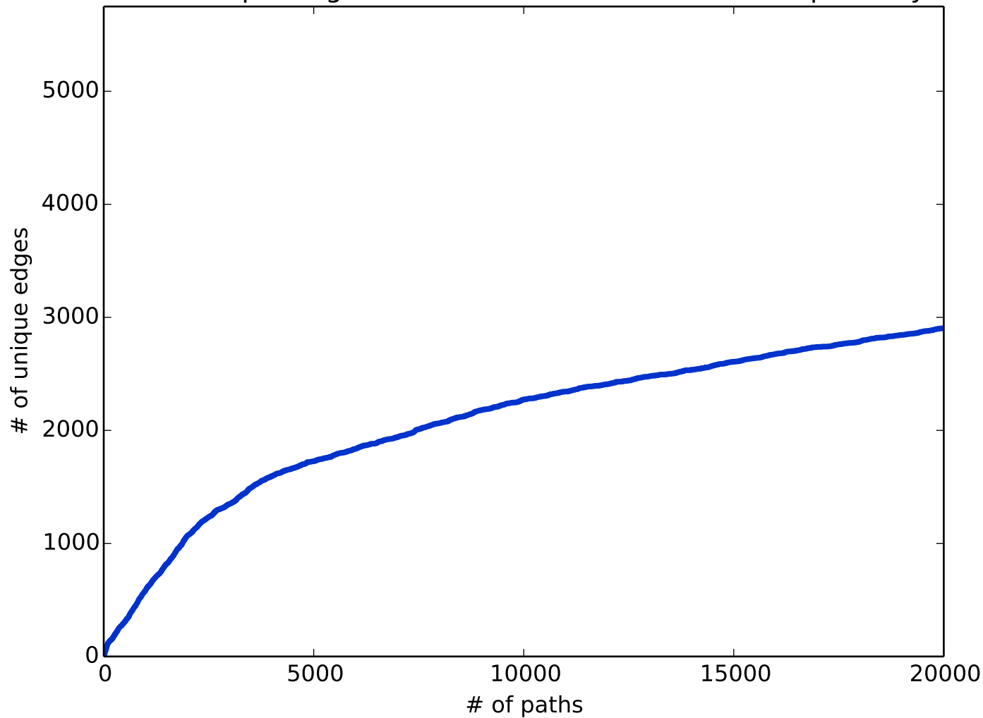
# of unique edges in the reconstruction of the IL6 pathway
