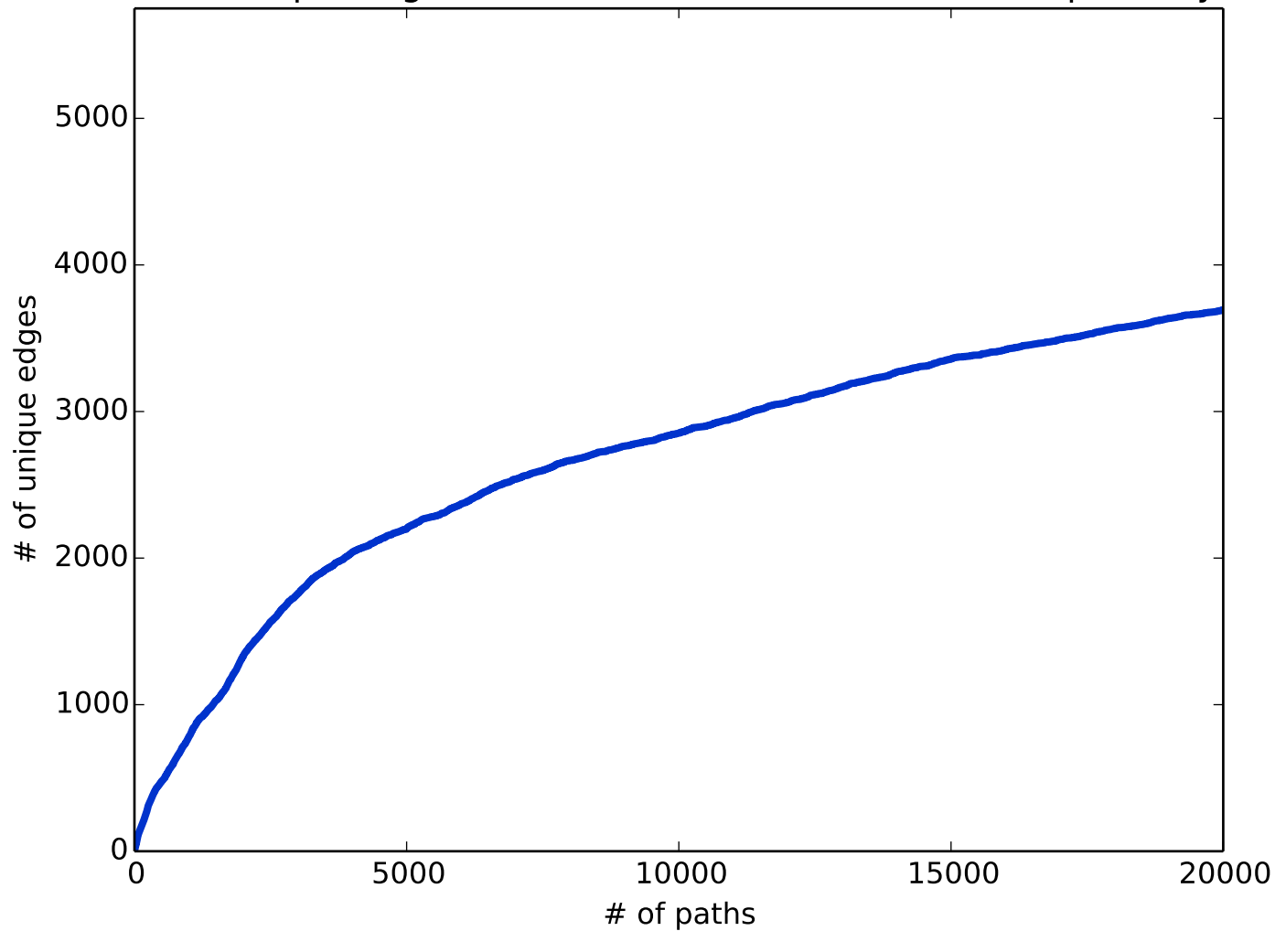
# of unique edges in the reconstruction of the \text{TNF}_\alpha pathway
