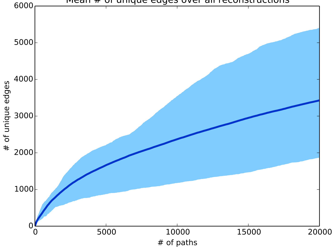
Mean # of unique edges over all reconstructions
