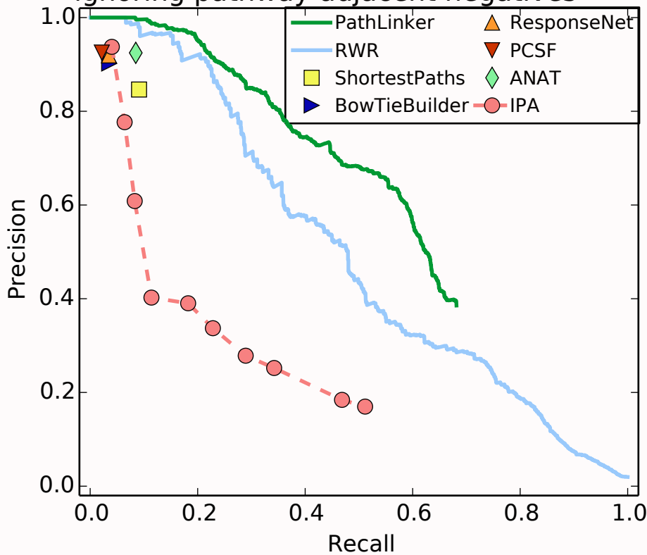
(b) Interactions aggregated over 15 pathway reconstructions, ignoring pathway-adjacent negatives
