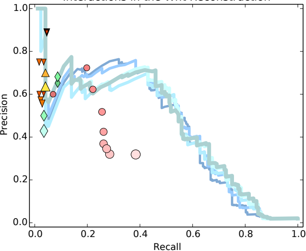
Interactions in the Wnt Reconstruction
