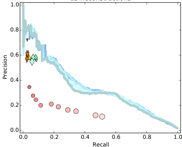
Interactions Aggregated over 15 Reconstructions
