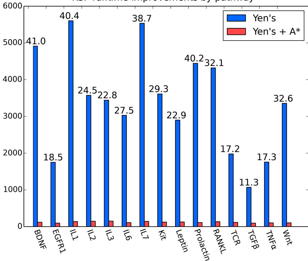
KSP runtime improvements by pathway
