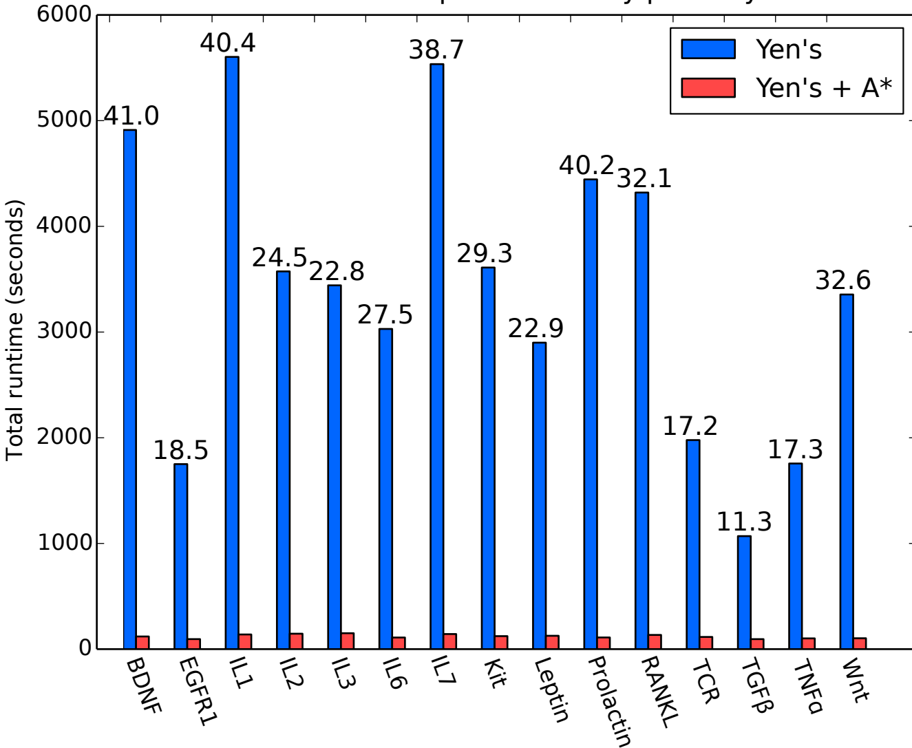
KSP runtime improvements by pathway
