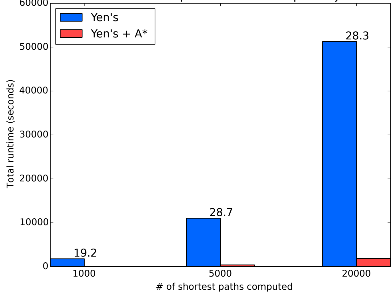
KSP runtime improvements over all pathways
