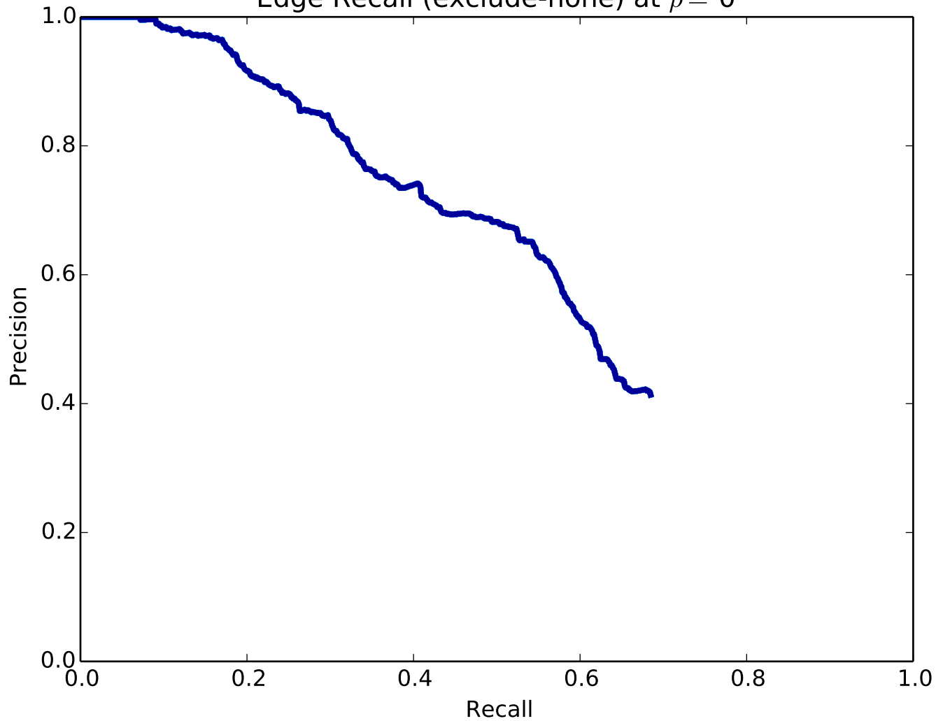
Edge Recall (exclude-none) at \rho = 0
