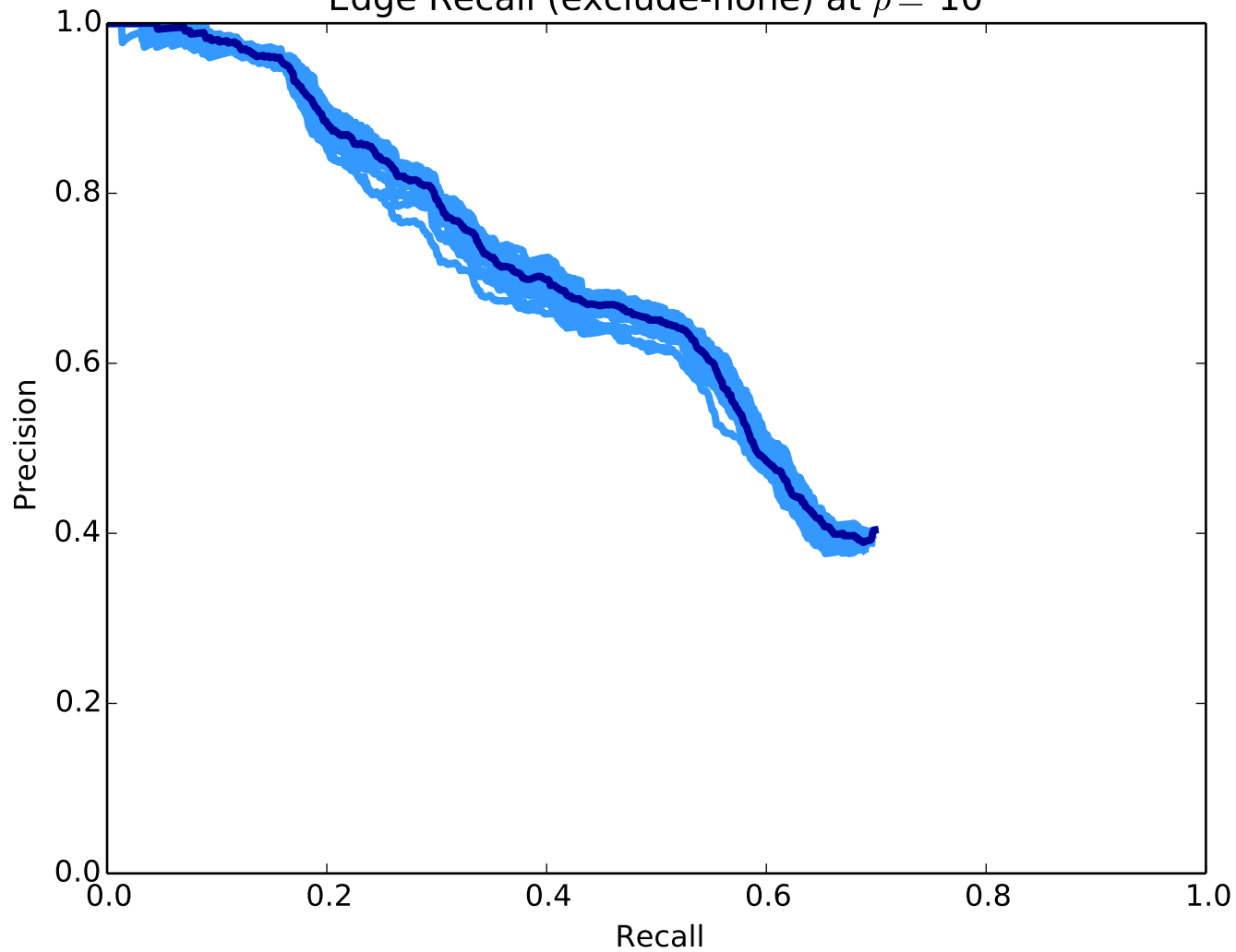
Edge Recall (exclude-none) at \rho = 10
