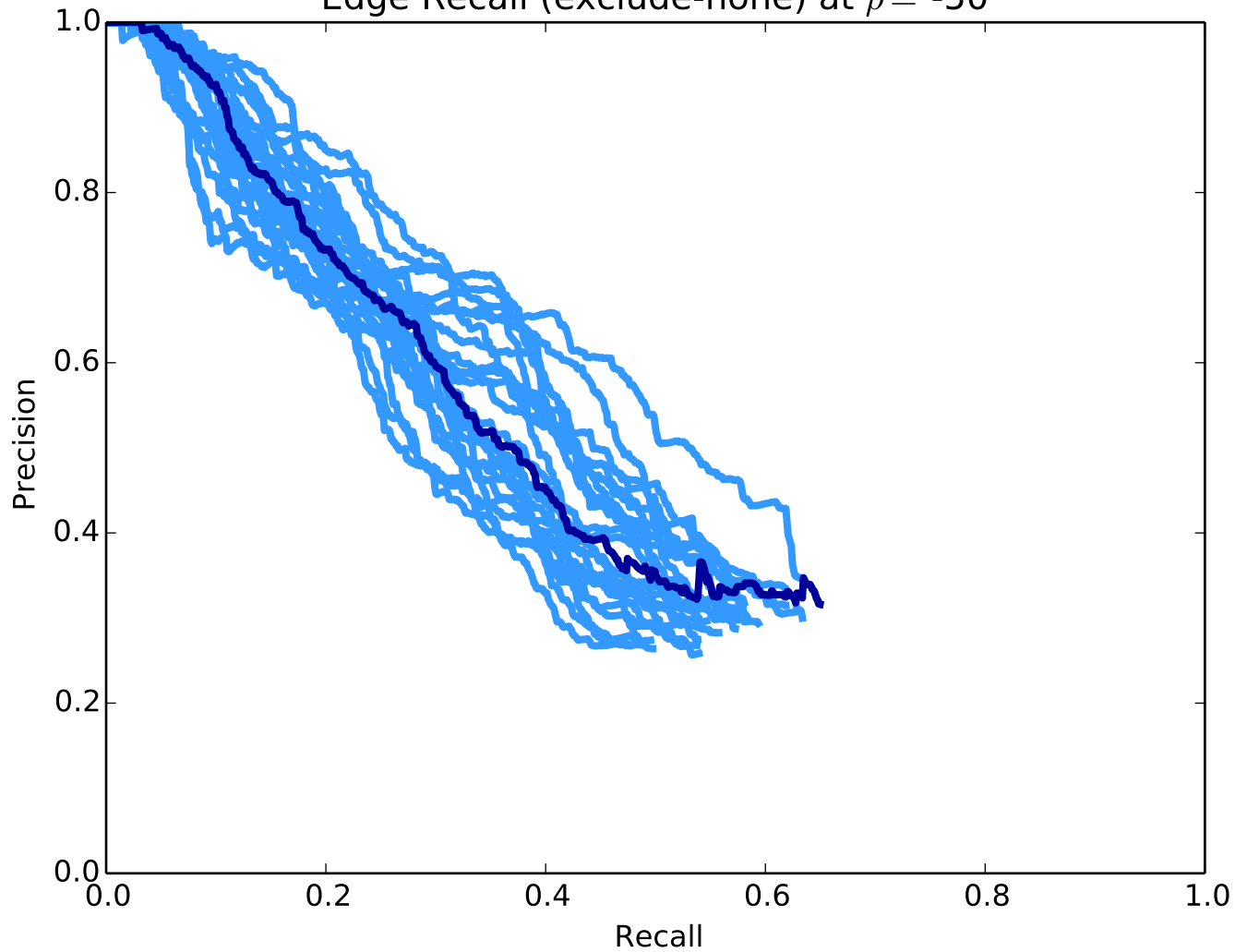
Edge Recall (exclude-none) at \rho = -50
