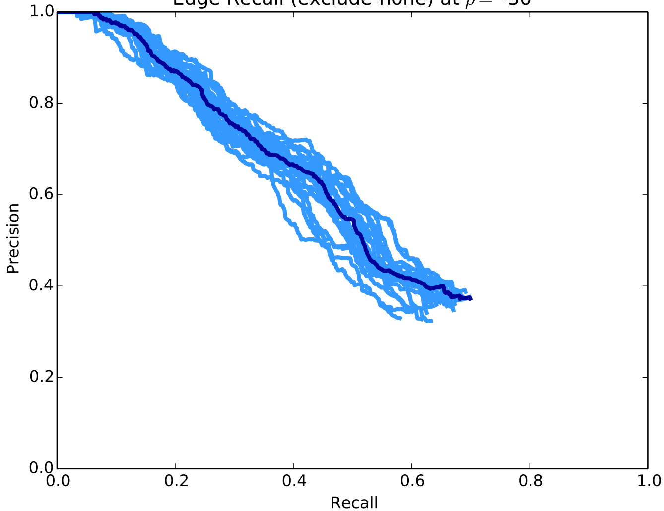
Edge Recall (exclude-none) at \rho = -30
