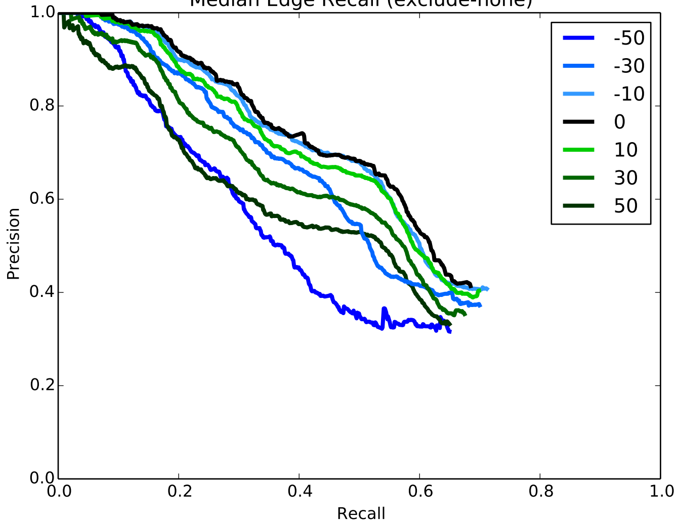
Median Edge Recall (exclude-none)
