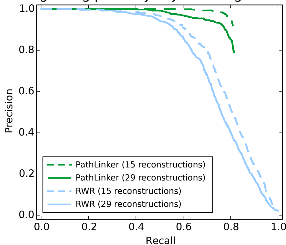
Interactions aggregated over NetPath reconstructions ignoring pathway-adjacent negatives
