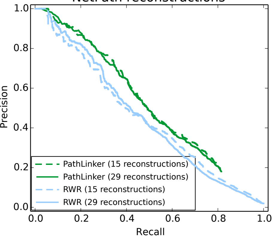
Proteins aggregated over NetPath reconstructions
