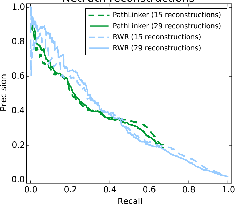
Interactions aggregated over NetPath reconstructions
