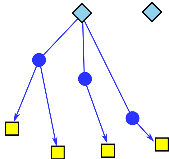
Succinct Sub-Networks
