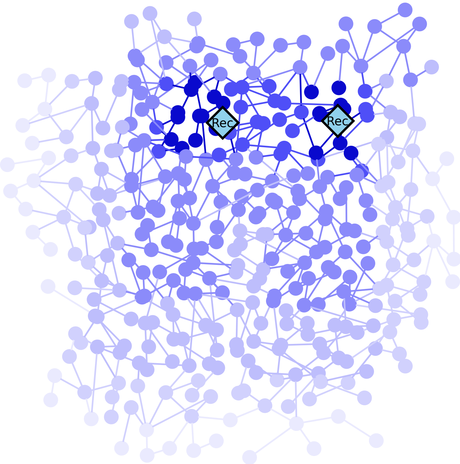
Weighted Interactome
