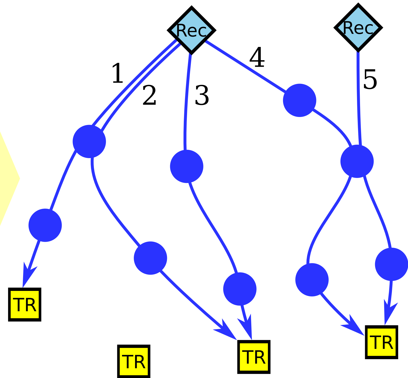
Computed Pathway
