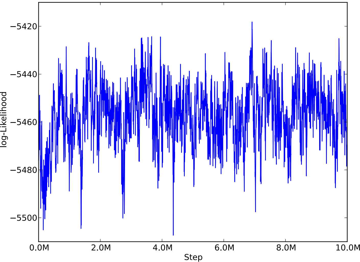
State log-Likelihood in progression through Markov chain
