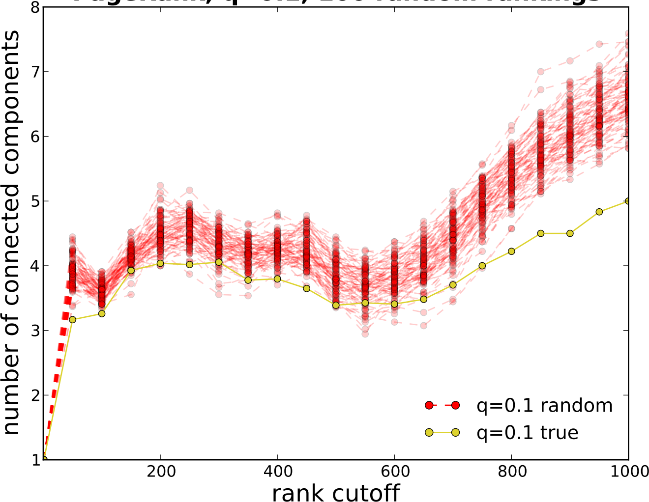
PageRank, q=0.1 , 100 random rankings
