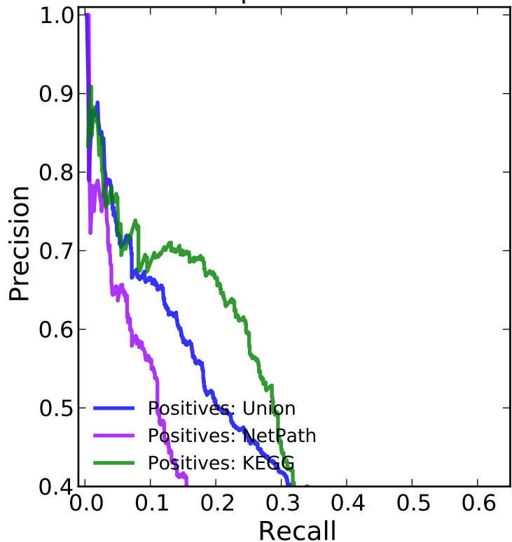
Aggregate Edge Prediction All Negatives Input: KEGG
