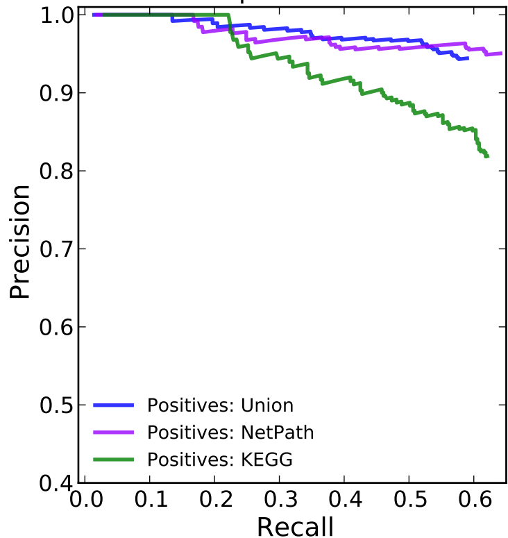
Aggregate Node Prediction Non-Adjacent Negatives Input: KEGG
