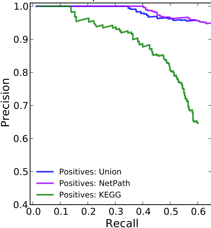
Aggregate Node Prediction Non-Adjacent Negatives Input: NetPath
