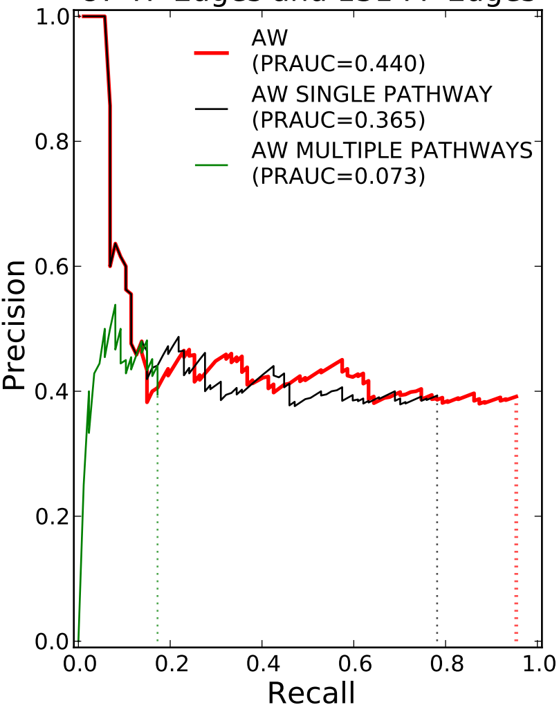
AW Highest Average Rank: k=1000 87 TP Edges and 131 FP Edges
