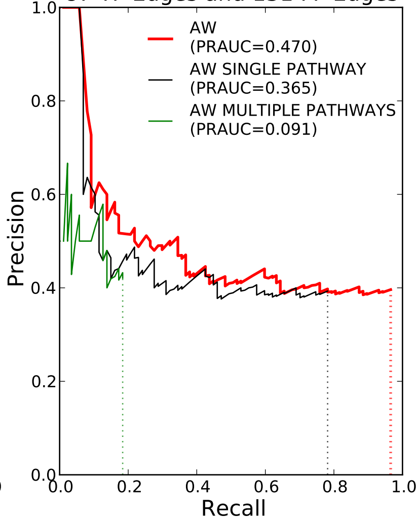
AW Highest Rank: k=1000 87 TP Edges and 131 FP Edges
