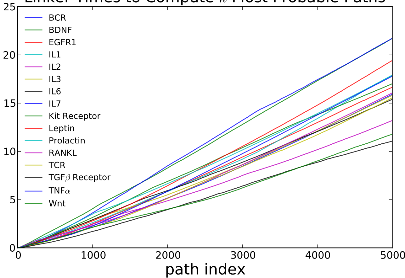
Linker Times to Compute k Most Probable Paths
