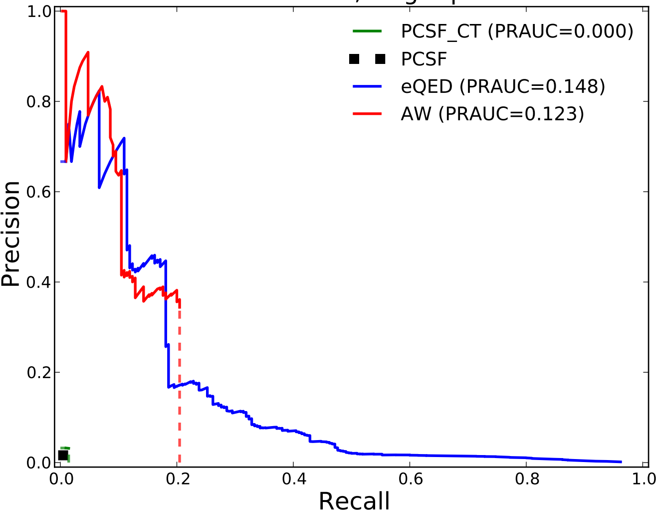
BCR true sources, target pool
