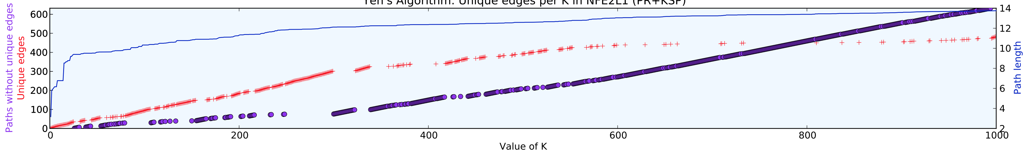
Yen's Algorithm: Unique edges per K in NFE2L1 (KSP)
