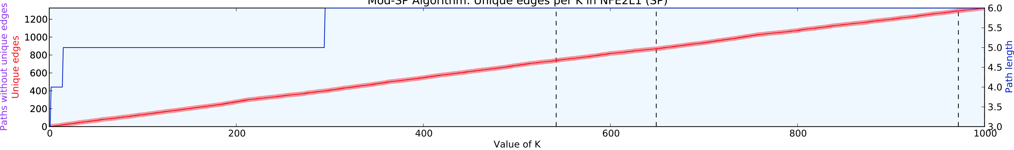
Mod-SP Algorithm: Unique edges per K in NFE2L1 (SP)
