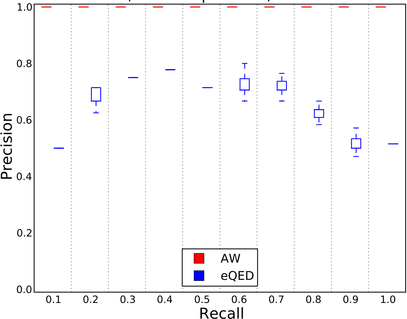
Embedded Pathway 4 level, 4 nodes per level, \lambda=0.0 noise
