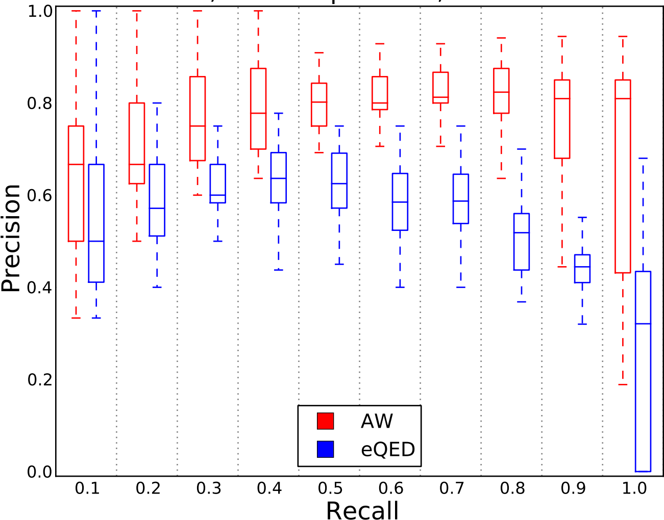
Embedded Pathway 4 level, 4 nodes per level, \lambda=0.2 noise
