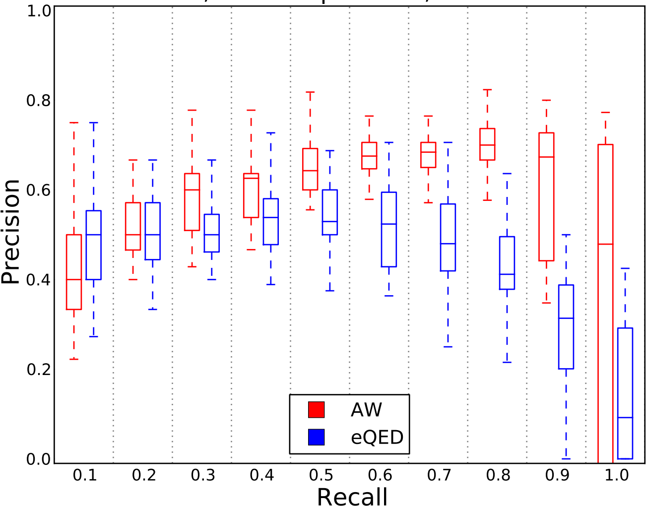
Embedded Pathway 4 level, 4 nodes per level, \lambda=0.5 noise
