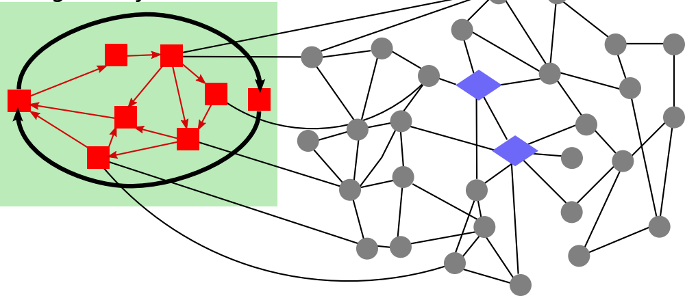
Cell cycle regulatory network
