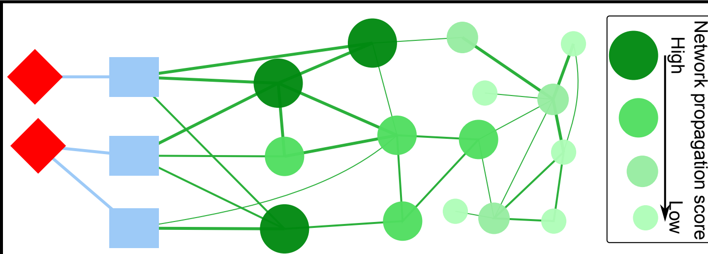
Network Propagation
