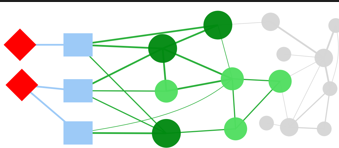
Top-ranking Proteins
