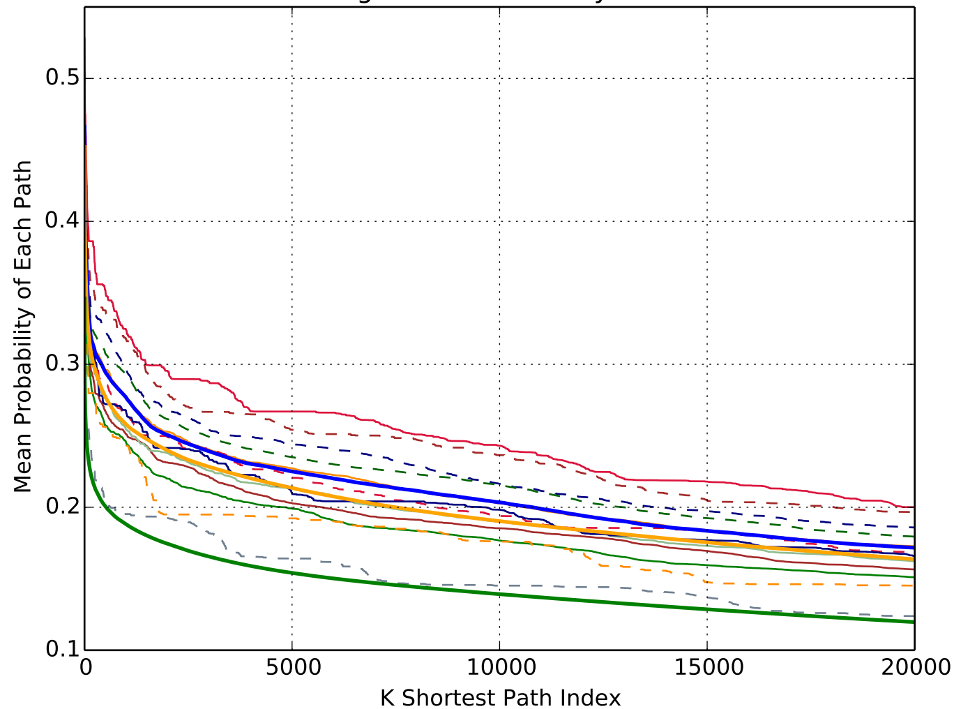
Average Path Probability k 20000
