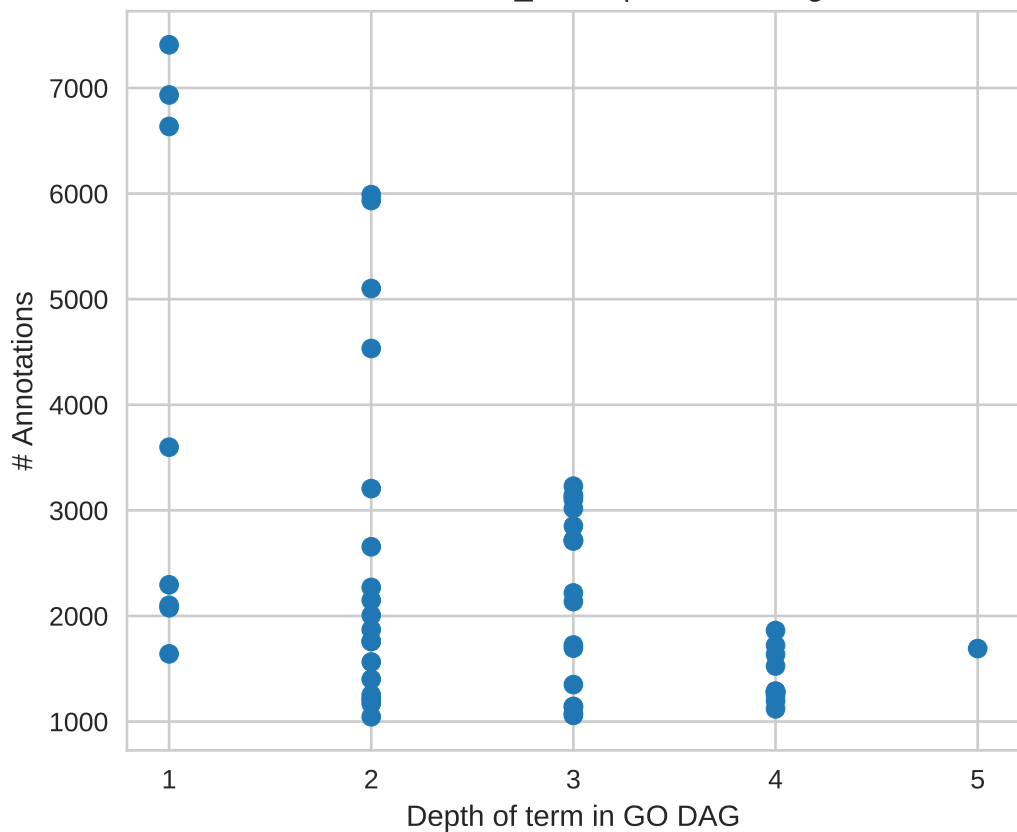
Depth of GO term in GO DAG by # of Annotations version: 2017_10-seq-sim-x5-string
