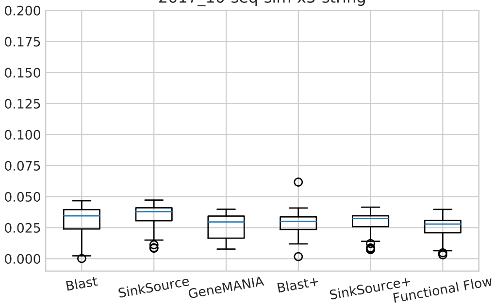
2017_10-seq-sim-x5-string
