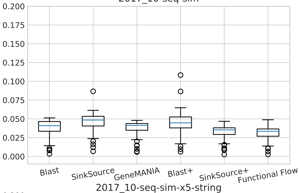
2017_10-seq-sim
