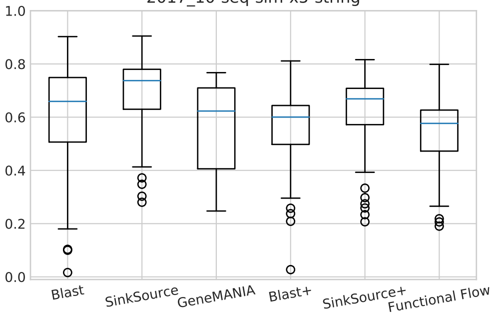
2017_10-seq-sim-x5-string
