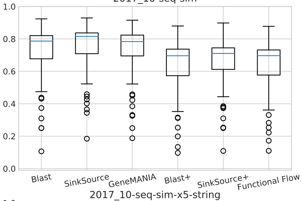
2017_10-seq-sim
