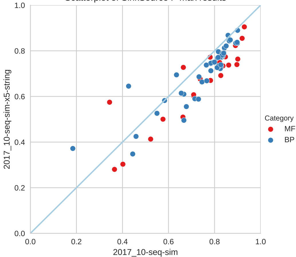
Scatterplot of SinkSource F-max results
