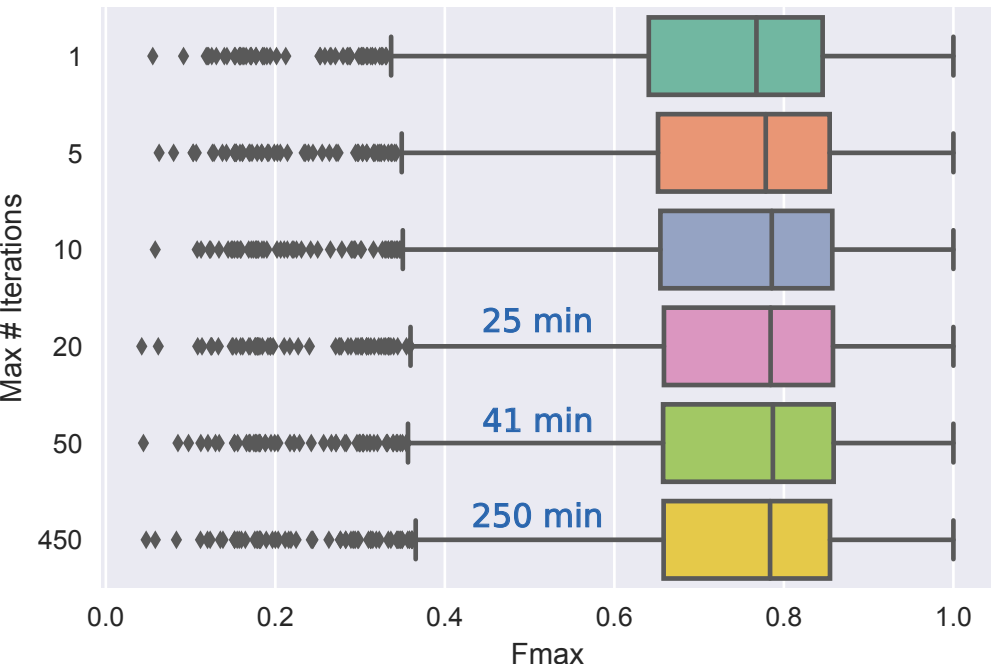
5 fold CV comparing # iterations 753 GO terms, SinkSource, alpha=0.8
