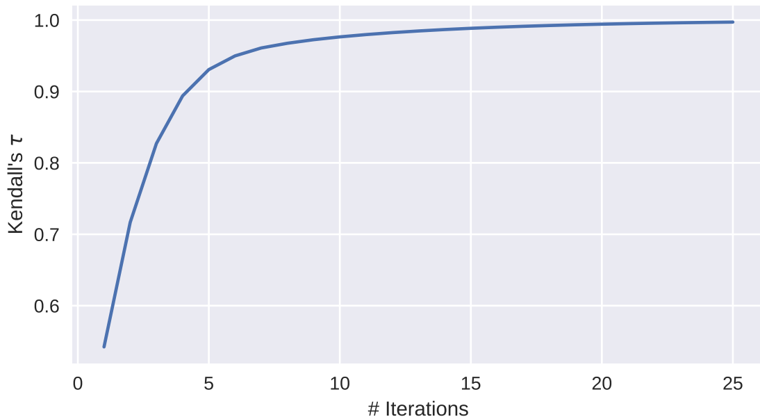
SinkSoucePlus-Squeeze comparison of node ranking to fixed ranking at each iteration Pathogenesis (GO:0009405) - all k
