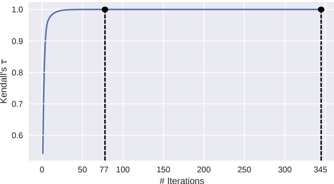
SinkSourcePlus Squeeze comparison of node ranking to fixed ranking at each iteration Pathogenesis (GO:0009405) all k
