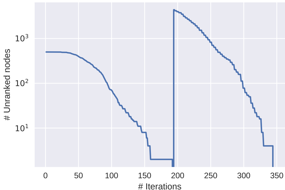
SinkSourcePlus-Squeeze number of nodes whose rank is not fixed by UB and LB Pathogenesis (GO:0009405) - all k
