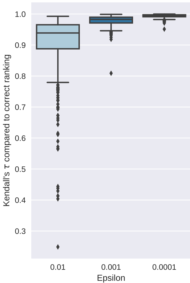
807 goterms, sinksource-squeeze, all k rem-neg-iea-50-1000
