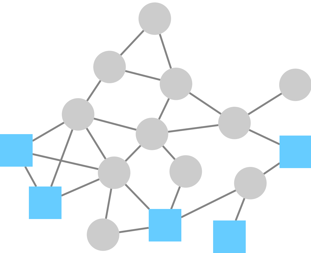
Original network
