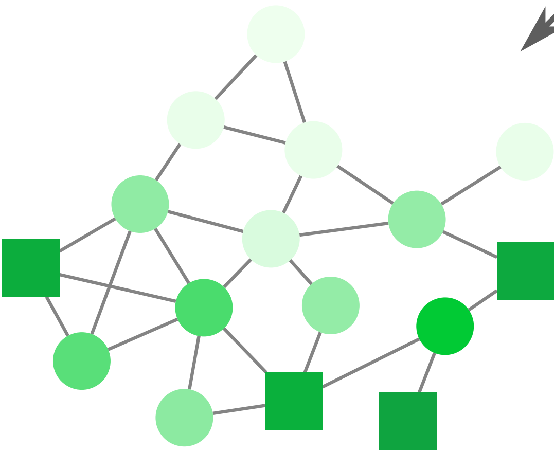
Network propagation
