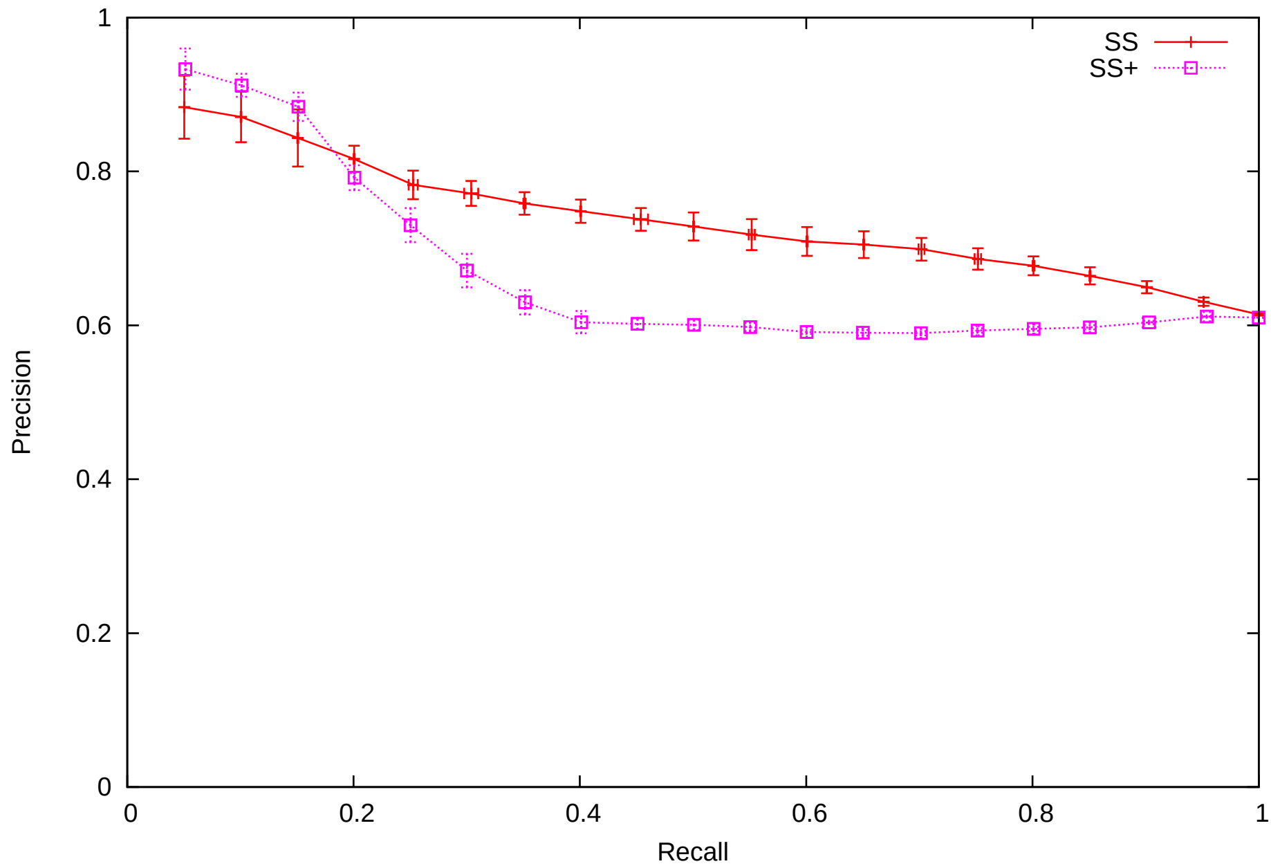
Brass-Konig-Zhou HDFs, MiMI unweighted network
