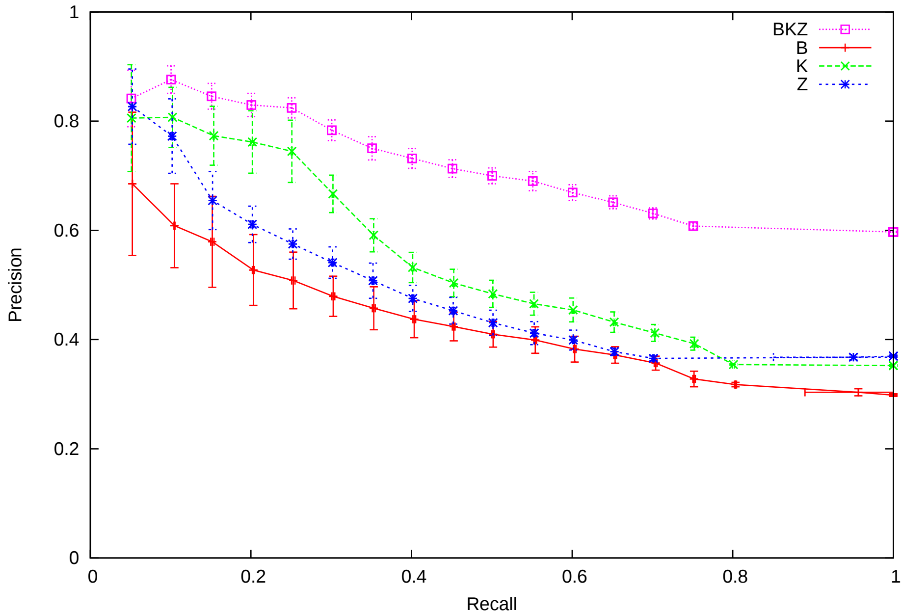
SinkSource, weighted network
