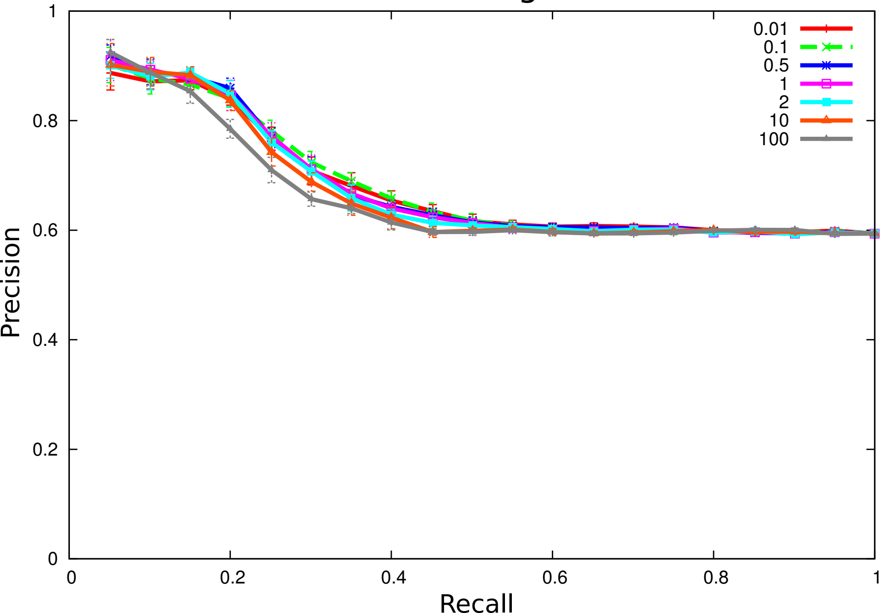
SinkSource+, unweighted network
